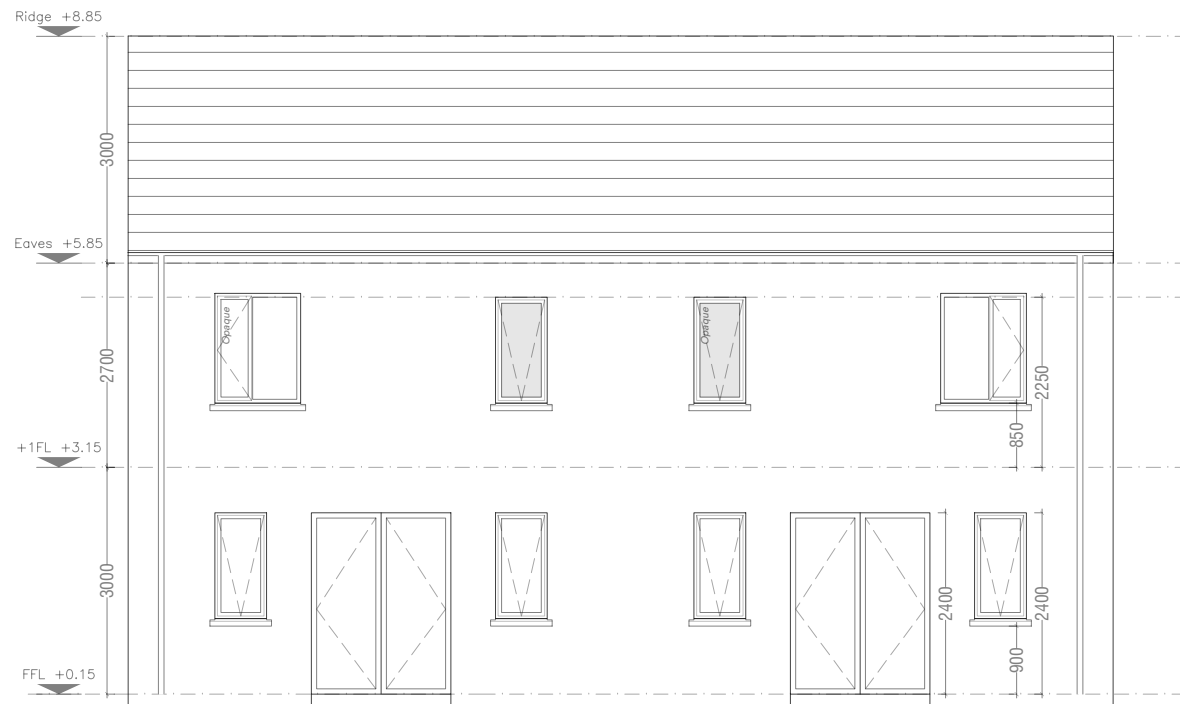
House Type K2 Semi-Detached Rear Elevation
