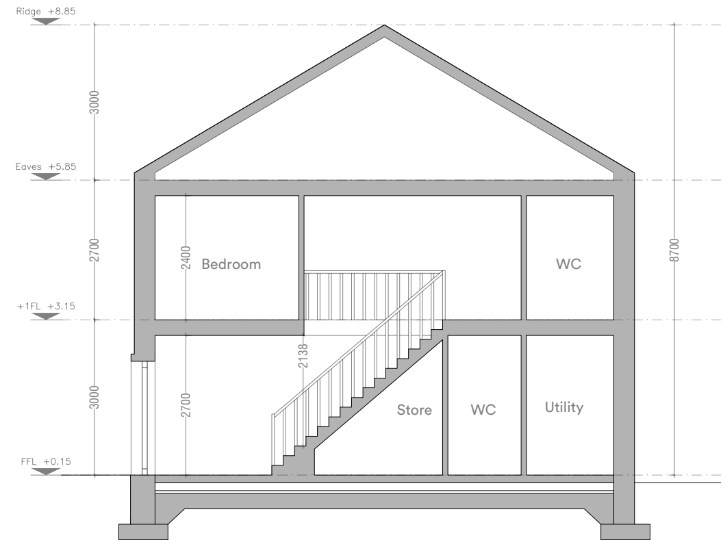
House Type K2 Semi-Detached Section A.A
